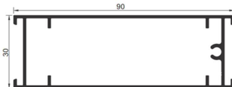
FCX-0218 – MONTANTE GIRO
